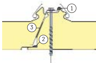
Joint detail, concealed fastening
