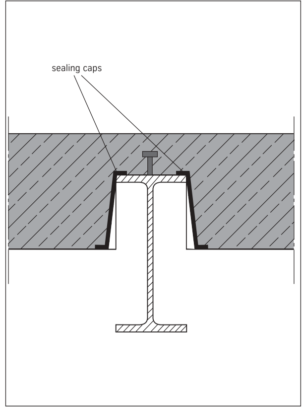
Intermediate supports
